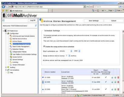
Archive stores management
