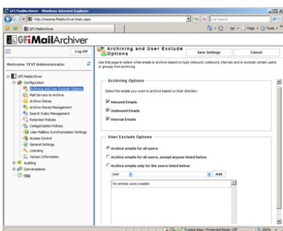
Archiving and user exclude options
